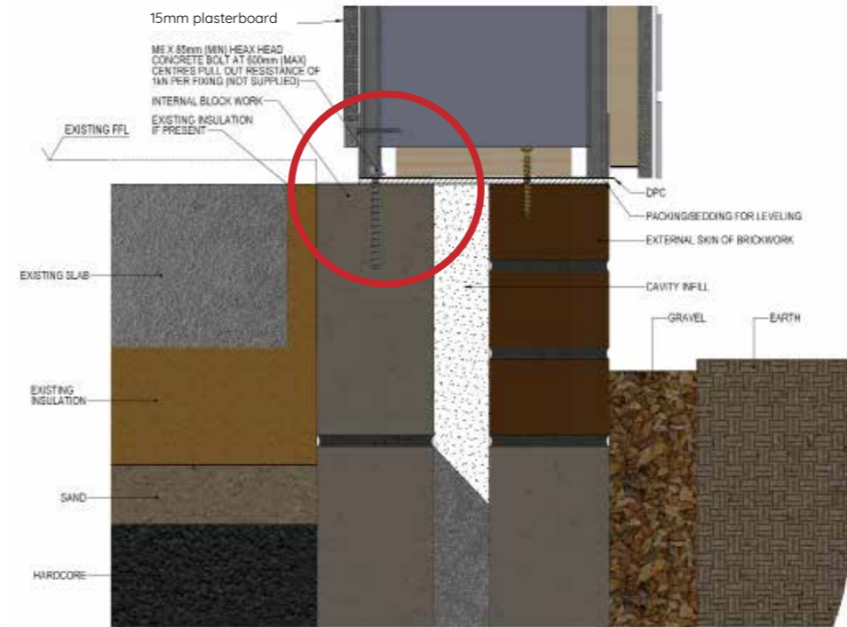
250mm Cavity Wall Base Detail (standard)
