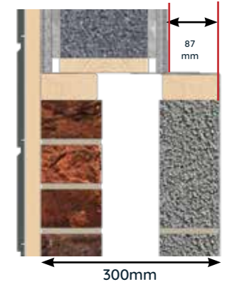
hup! on 300mm existing wall - full clad
