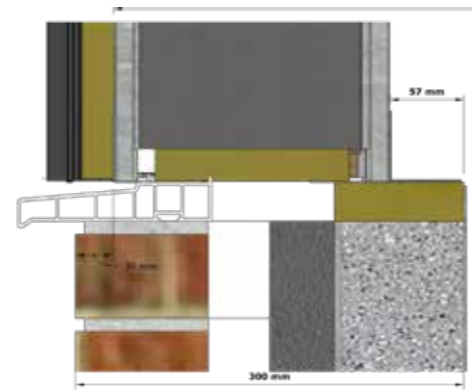
hup! on 300mm existing wall - on cill
