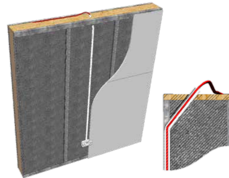
Drill hole through top tray and EPS to thread conduit through.
