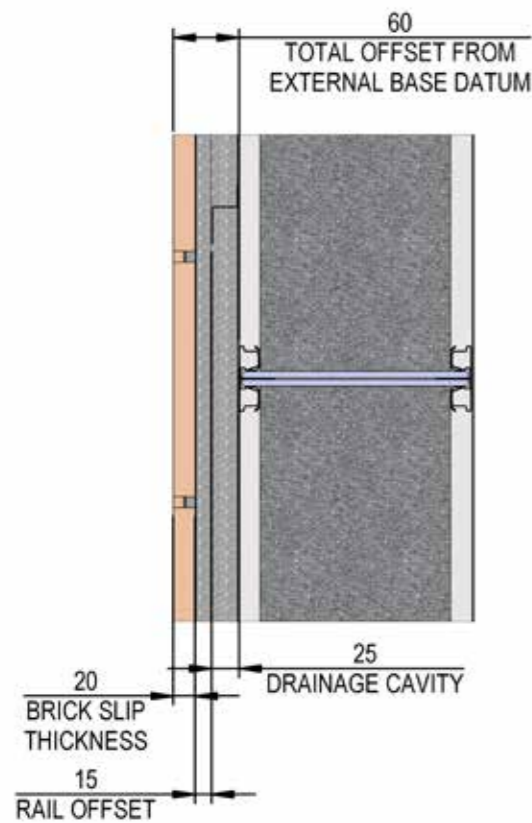
hup! walls with brick slips rails
