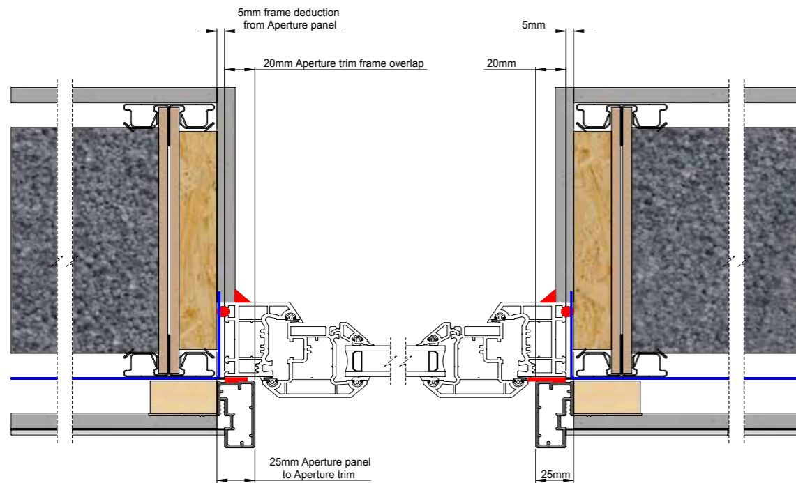
Small frames may require 20mm add ons to avoid opening sashes fouling on the aperture trim, or for aesthetic reasons
