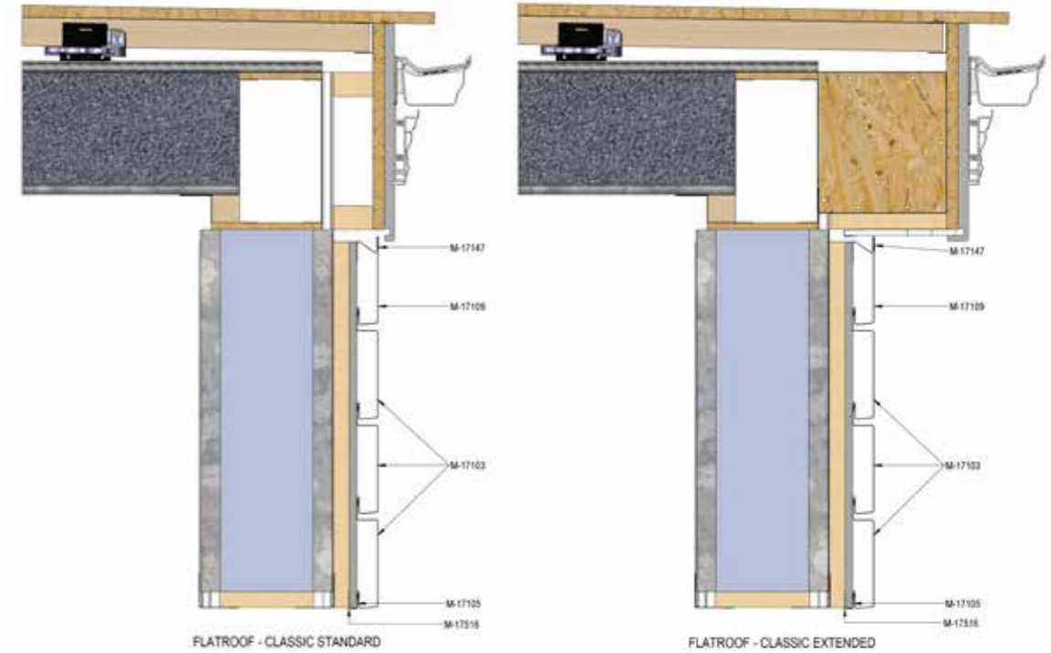
Flat Roof classic with steel facade
